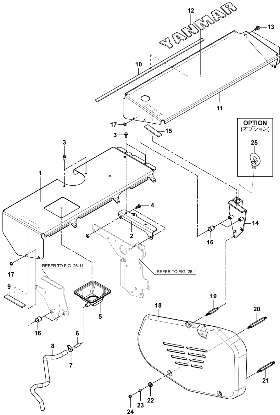
Fig.43. TOP COVER & V-BELT COVER
