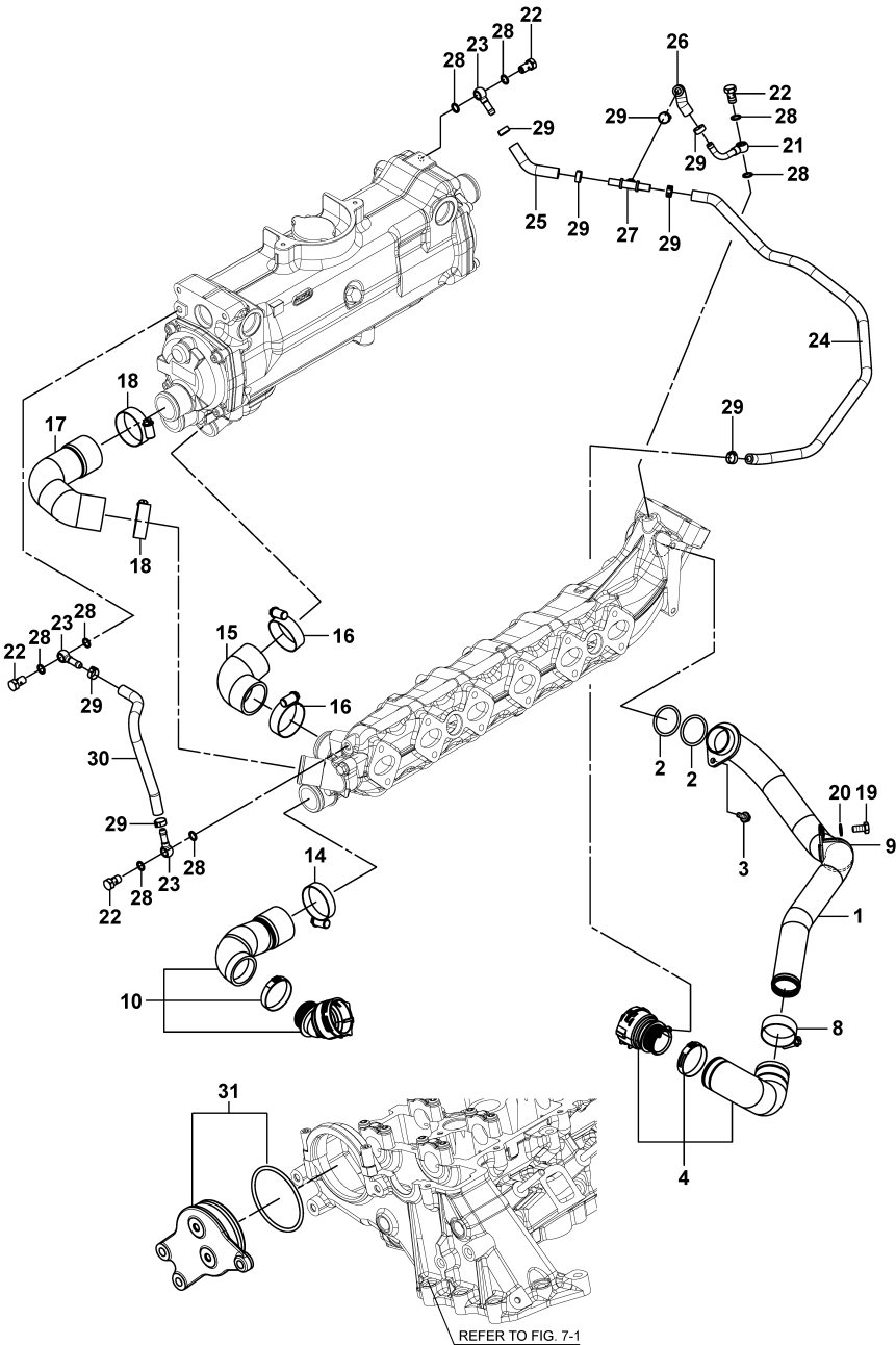
Fig.28. HOSE, FW PUMP
