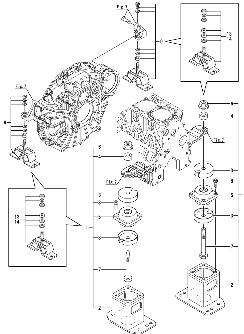
Fig.60. FLEXIBLE MOUNT
