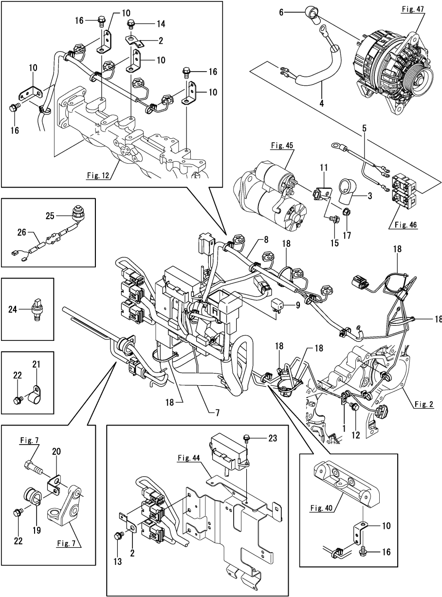
Fig.49. WIRE HARNESS
