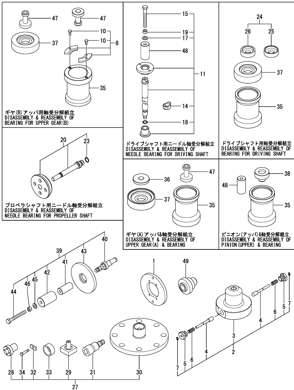
Fig.11. SPECIAL TOOL(B)(OPTIONAL)
